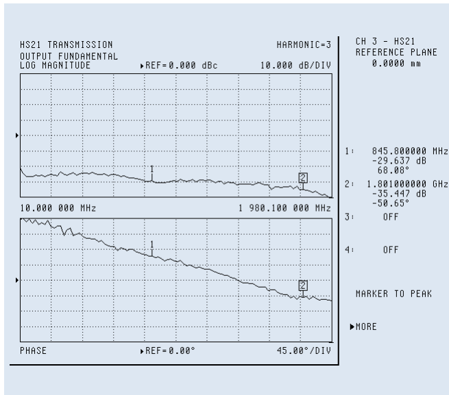
Figure 6. The 3 rd harmonic (magnitude and phase) of an example amplifier under fully calibrated conditions is shown here. This amplifier was driven with +5 dBm and had a 10 dB pad on the output to minimize non-linear receiver effects. A 10 Hz IFBW was used during measurement and calibration.
