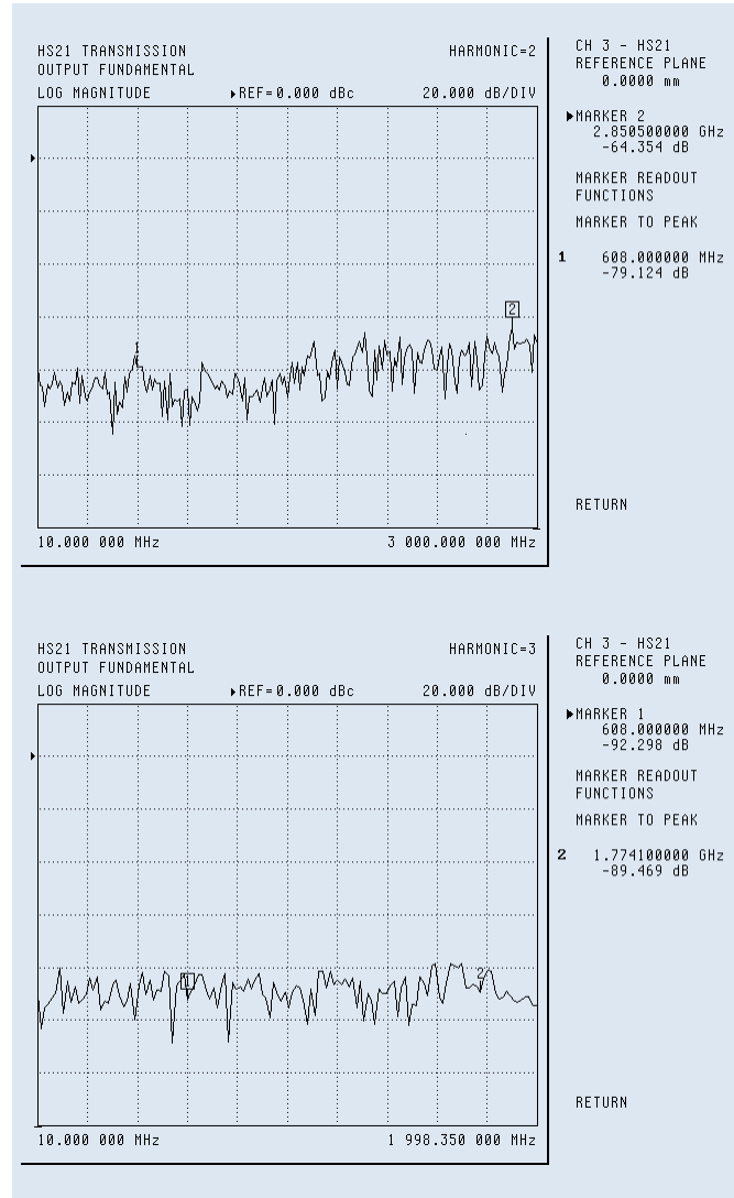
Figure 4. Example dynamic range plots under ENHANCEMENT cal for both 2 nd and 3 rd harmonics are shown here. The calibration and measurement power is +0 dBm. The measurement is performed with the same thru line in place as was used during the cal.
