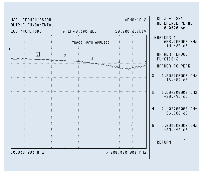
Figure 2. The 2 nd harmonic of a sample amplifier in SOURCE swept mode. The trace data is divided by a normalization (obtained with harmonic = 1) so the displayed values are relative to the fundamental. Note that the reference level will always be labeled "dBc" with an absolute power reference, a reference to the fundamental carrier, or no reference at all. The user must interpret the displayed values as appropriate.
