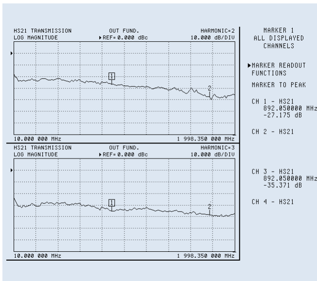
Figure 5. A two channel plot showing the 2 nd and 3 rd relative harmonic levels of an amplifier using the ENHANCEMENT calibration state. The cal and measurement were performed with a source power of +0 dBm and the amplifier output was padded to avoid receiver compression.
