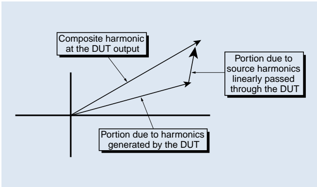
Figure 3. An illustration of the composition of the harmonic signal at the DUT output assuming the source harmonics are not so large as to affect the DUT's operating state.
