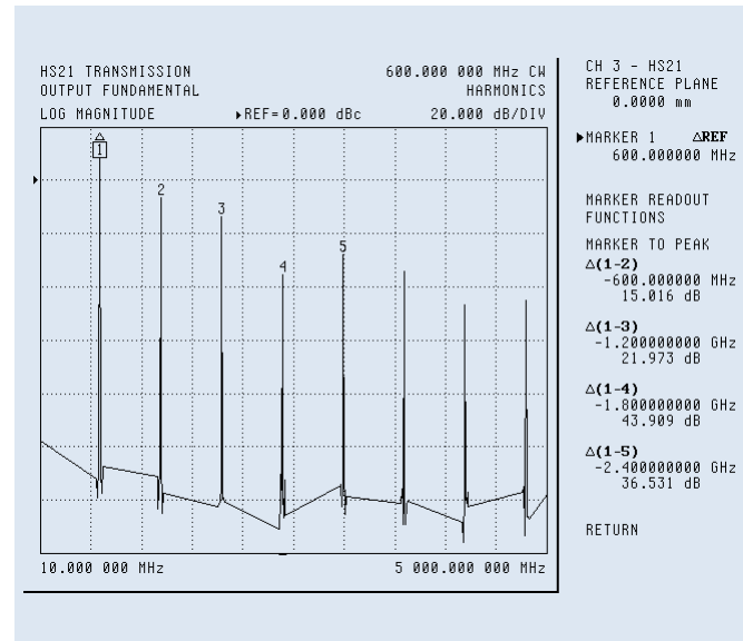
Figure 1. A plot in CW RCVR mode of the harmonics of a sample amplifier. The relative harmonic levels are displayed via marker reference. The source in this case is at 600 MHz and the first 8 harmonics are displayed.
